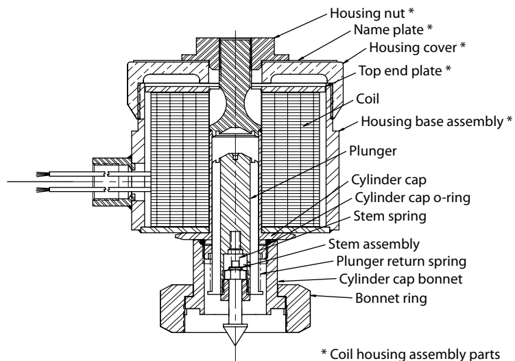
* Coil housing assembly parts Explosion-proof NEMA 7 & 9 coil housing option (Shown with a DC coil) for the following valve series: 13000, 30400, 30800, 35000, 40000, and 50000
